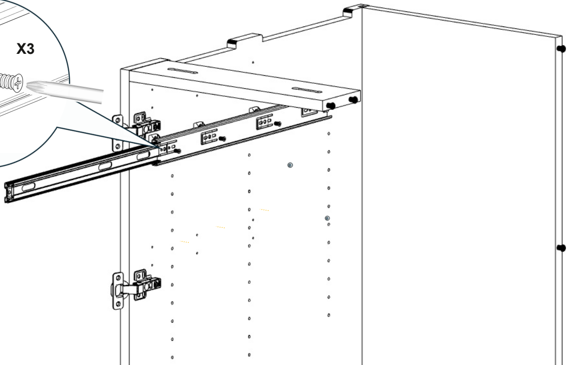
Step 4: Fully extend the Cabinet Box Rail and attach it to the Drawer Glide Spacers on the left Side Panel using (3) 5 mm Euro screws, as shown. Repeat on the Right Side Panel.
